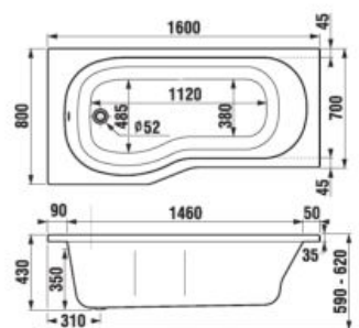
built-in version
