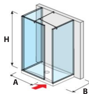
glass wall/walk in PURE for shower trays 70, 80 × 80 cm | 70, 80 × 90 cm
